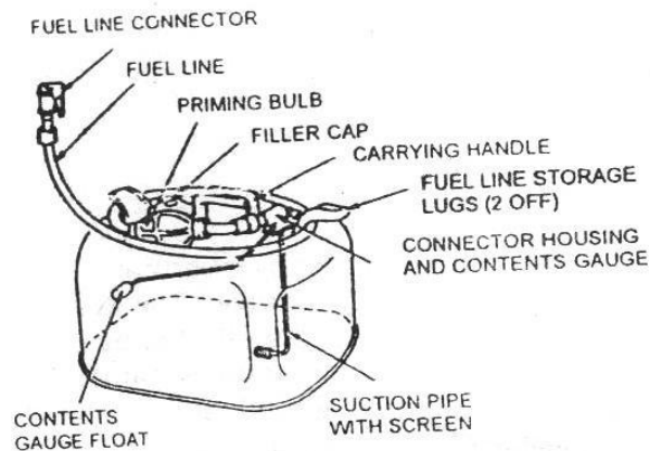
Fuel Tank and Fittings
